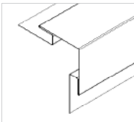
OUTSIDE CORNER
